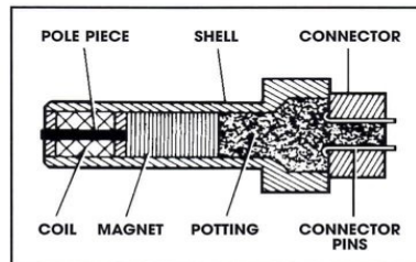
Cut-A-Way View of VRS Magnetic Sensor
