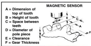
Optimum Gear Tooth Configuration
