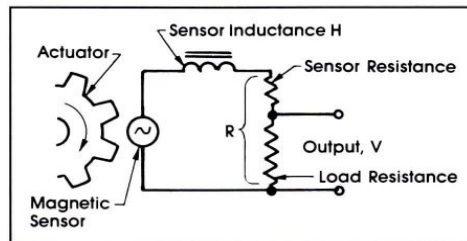
Equivalent Circuit
