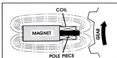
High Reluctance Position of Magnetic Circuit
