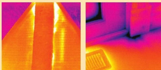
Figure 4. Inspecting to locate air leakage requires a 4 °F or higher temperature difference between inside and outside air, in order to get accurate readings. Air leakage can be into the building, as in the cold air shown leaking through the floor, or out of it, as in the warm air leaking out alongside the chimney. Images courtesy of Snell Infrared ©2005.
