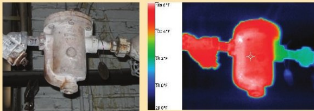
Figure 7. When operating correctly, as in this example, steam trap thermal images should show an abrupt change in temperature.
