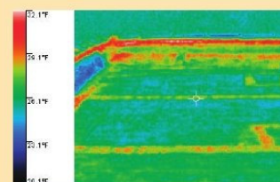
Figure 5. Cool areas on this roof exposure probably indicate moisture buildup. Mark with tape and investigate with core samples.
