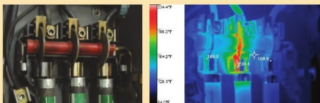
Figure 2. Fused power disconnect and corresponding infrared image.
