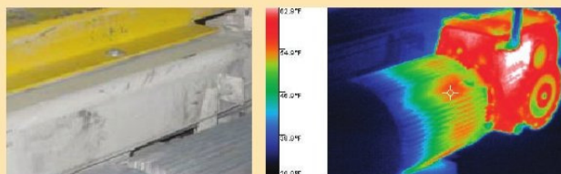
Figure 6. This thermal image shows a cool motor on the left and a hot gearbox on the right, with an especially white-hot anomaly.
